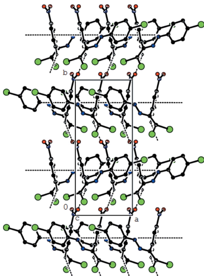
Figure 4 View down the c -axis of the C-H\cdots O and \pi-\pi interactions (dashed lines) in the title compound.
