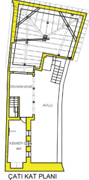
ÇATI KAT PLANI
