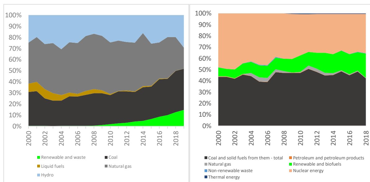
Figure 1. Electricity production in Turkey (left) and Bulgaria (right), according to the sources
