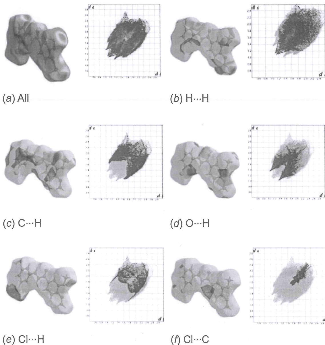
Figure 4 Hirshfeld surface of the title complex plotted over shape-index.
