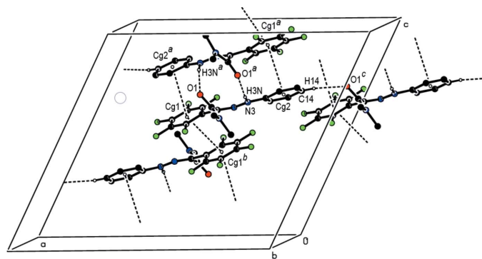
Figure 2 View oblique to [010] of the intermolecular N-H\cdots O , C-H\cdots O and \pi-\pi stacking interactions of the title compound.
