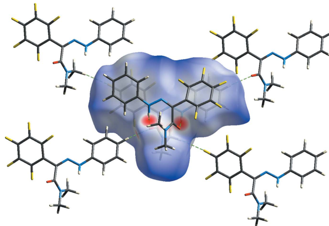
Figure 3 View of the three-dimensional Hirshfeld surface of the title compound plotted over d_{\text{norm}} in the range –0.52 to 2.23 a.u.
