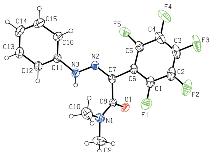
Figure 1 The title molecule showing 30% probability displacement ellipsoids.
