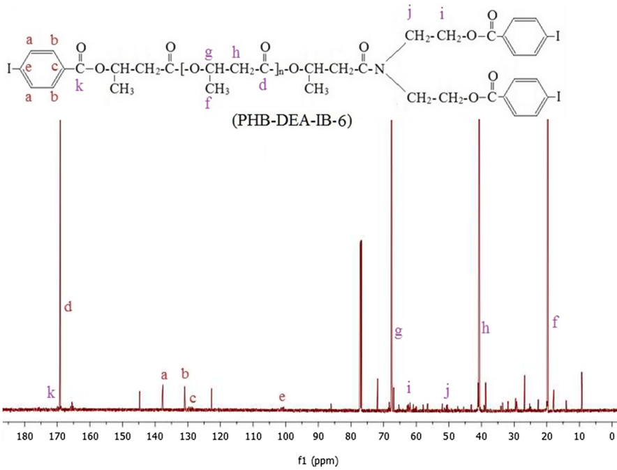
Fig. 3 13 C NMR spectrum of the iodinated PHB sample containing 4-iodobenzoyl groups (PHB-DEA-IB-6)
